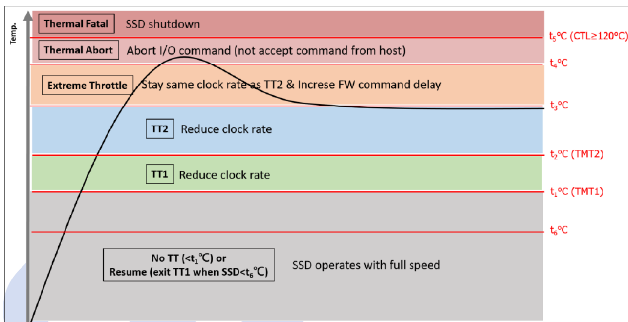
Figure 2-1 Thermal Throttling Schematic
